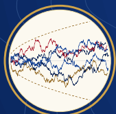
WIENER PROCESS
