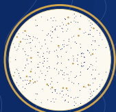
ELLIPTIC CURVES
