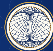
MODULAR ARITHMETIC
