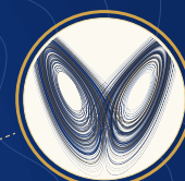
STRANGE ATTRACTORS
