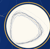
STOCHASTIC DELAY
